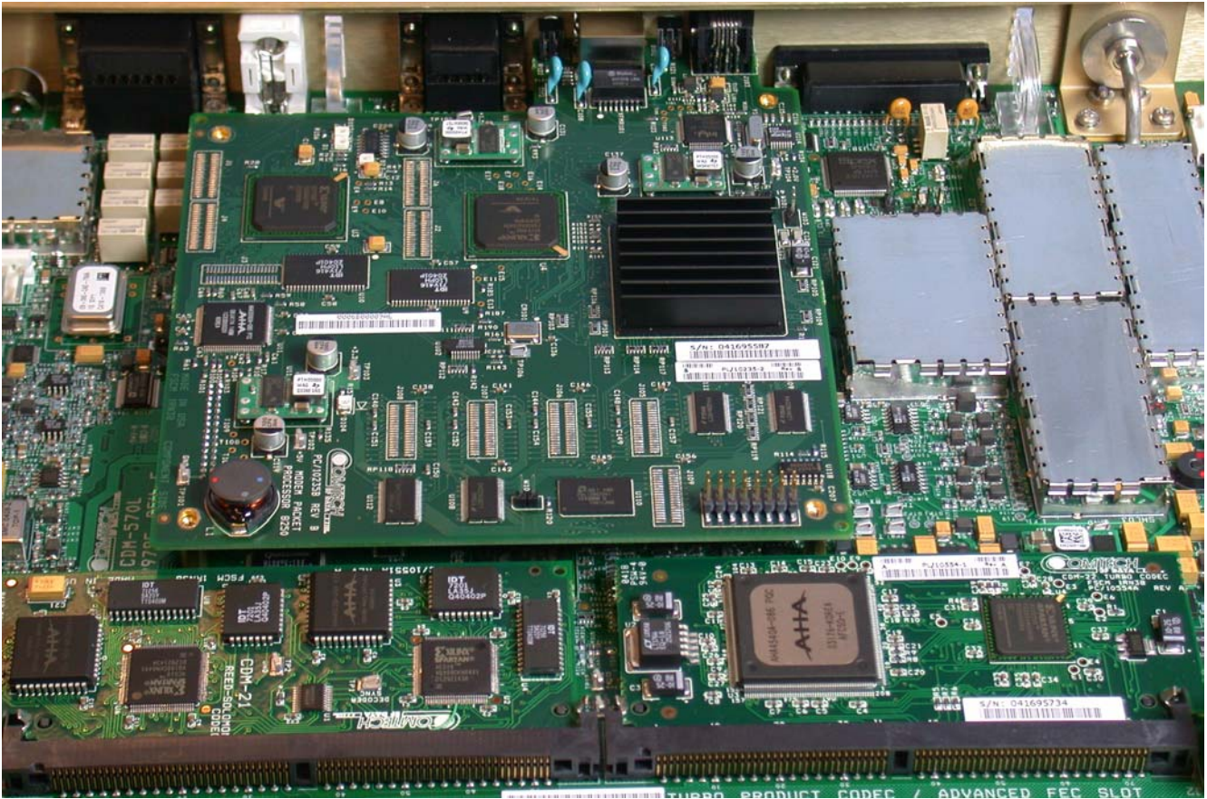
Figure 5. MPP50 board properly installed in the CDM-570L Modem
